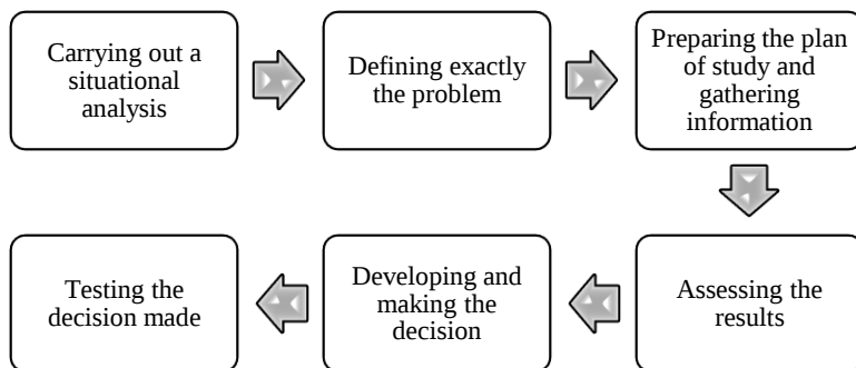
Fig 2. “SELECT” Model
